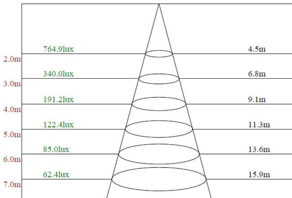
Beam angle of C90plane97.16
