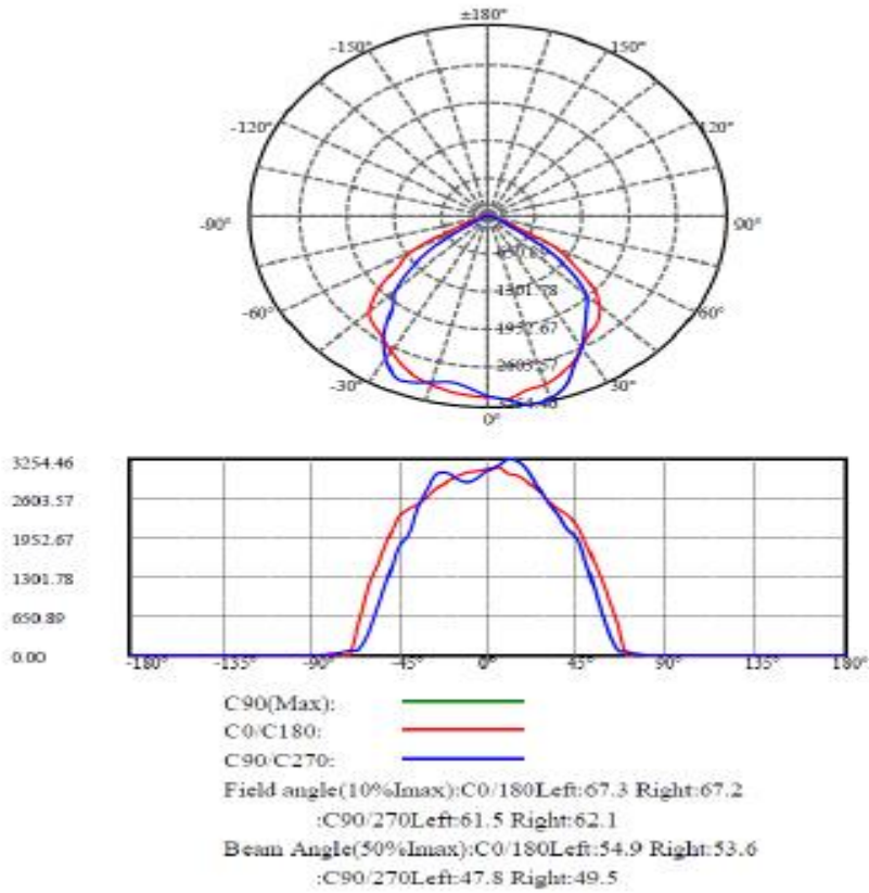
Light Distribution Curve [Unit: cd]
